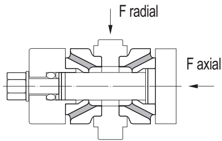
TYPICAL FITTING ARRANGEMENT
